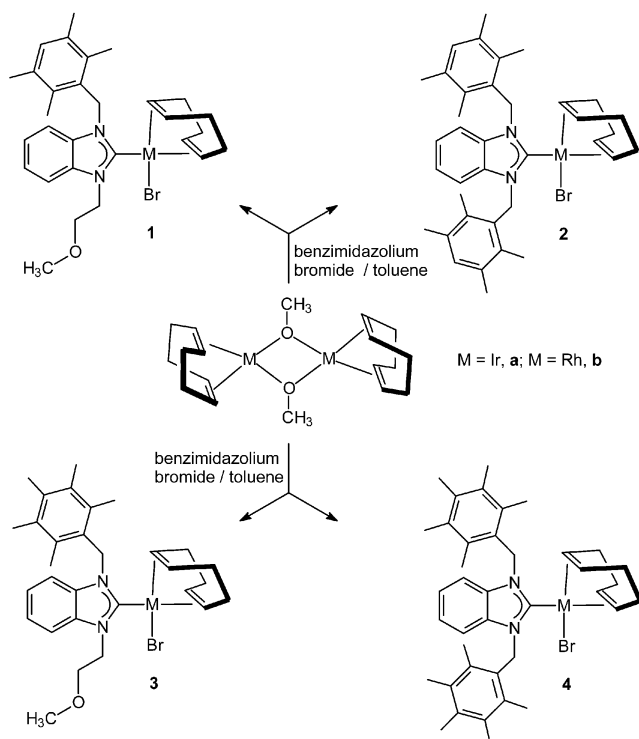
Scheme 1. Preparation of \text{Rh}^{\text{I}} and \text{Ir}^{\text{I}} complexes 1–4 .
