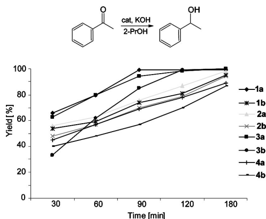
Figure 4. Time dependence of the catalytic transfer hydrogenation of acetophenone; catalyst ( 1a–4b , 0.02 mmol), KOH (0.2 mmol), acetophenone (4 mmol), and 2-propanol (20 mL), T = 353 K.
