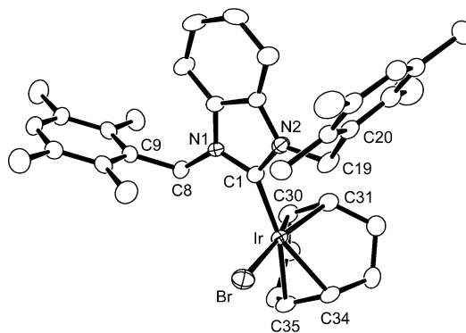
Figure 2. Molecular structure of complex 2a in 2\text{a} \cdot \text{CH}_2\text{Cl}_2 (hydrogen atoms have been omitted). Selected bond lengths [Å] and angles [°]: \text{Ir}-\text{Br} 2.4803(6), \text{Ir}-\text{C1} 2.010(4), \text{Ir}-\text{C30} 2.109(5), \text{Ir}-\text{C31} 2.117(5), \text{Ir}-\text{C34} 2.195(5), \text{Ir}-\text{C35} 2.192(5), \text{N1}-\text{C1} 1.363(6), \text{N2}-\text{C1} 1.361(6), \text{C30}-\text{C31} 1.406(7), \text{C34}-\text{C35} 1.390(7); \text{Br}-\text{Ir}-\text{C1} , 90.75(13), \text{Br}-\text{Ir}-\text{C30} 161.58(14), \text{Br}-\text{Ir}-\text{C31} 159.42(14), \text{Br}-\text{Ir}-\text{C34} 93.12(14), \text{Br}-\text{Ir}-\text{C35} 89.61(14), \text{C1}-\text{Ir}-\text{C30} 93.3(2), \text{C1}-\text{Ir}-\text{C31} 88.1(2), \text{C1}-\text{Ir}-\text{C34} 158.4(2), \text{C1}-\text{Ir}-\text{C35} 164.5(2), \text{C30}-\text{Ir}-\text{C31} 38.9(2), \text{C30}-\text{Ir}-\text{C34} 89.7(2), \text{C30}-\text{Ir}-\text{C35} 81.7(2), \text{C31}-\text{Ir}-\text{C34} 80.9(2), \text{C31}-\text{Ir}-\text{C35} 96.9(2), \text{C34}-\text{Ir}-\text{C35} 36.9(2), \text{N1}-\text{C1}-\text{N2} 105.9(4).
