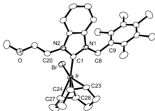
Figure 3. Molecular structure of complex 3a (hydrogen atoms have been omitted). Selected bond lengths [Å] and angles [°]: Ir–Br 2.4907(5), Ir–C1 1.999(4), Ir–C23 2.110(4), Ir–C23 2.118(4), Ir–C27 2.195(4), Ir–C28 2.197(4), N1–C1 1.367(5), N2–C1 1.361(4), C23–C24 1.422(6), C27–C28 1.385(6); Br–Ir–C1, 87.46(10), Br–Ir–C23 158.70(11), Br–Ir–C24 161.96(12), Br–Ir–C27 91.12(12), Br–Ir–C28 93.48(11), C1–Ir–C23 90.78(14), C1–Ir–C24 94.85(15), C1–Ir–C27 163.4(2), C1–Ir–C28 159.9(2), C23–Ir–C24 39.33(15), C23–Ir–C27 96.4(2), C23–Ir–C28 81.07(15), C24–Ir–C27 81.6(2), C24–Ir–C28 90.5(2), C27–Ir–C28 36.8(2), N1–C1–N2 105.7(3).
