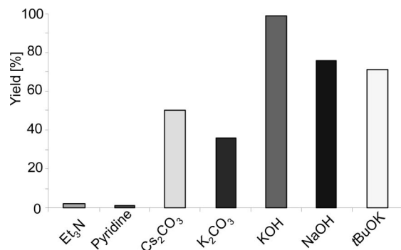
Figure 6. Influence of the base on the transfer hydrogenation of acetophenone by using catalyst 1a (0.02 mmol), acetophenone (4 mmol), and 2-propanol (20 mL), T = 353 K, t = 90 min.
