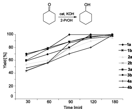
Figure 5. Time dependence of the catalytic transfer hydrogenation of cyclohexanone; catalyst ( 1a–4b , 0.02 mmol), KOH (0.2 mmol), cyclohexanone (4 mmol), and 2-propanol (20 mL), T = 353 K.
